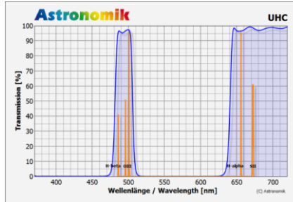
Narrowband Filter
