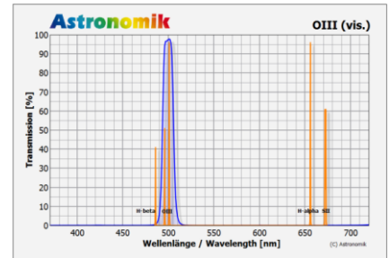
Line Filter
