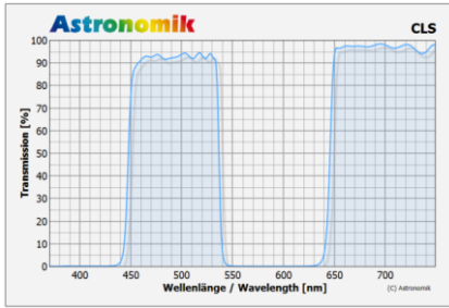
Broadband Filter
