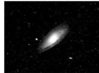
DARK SKY
