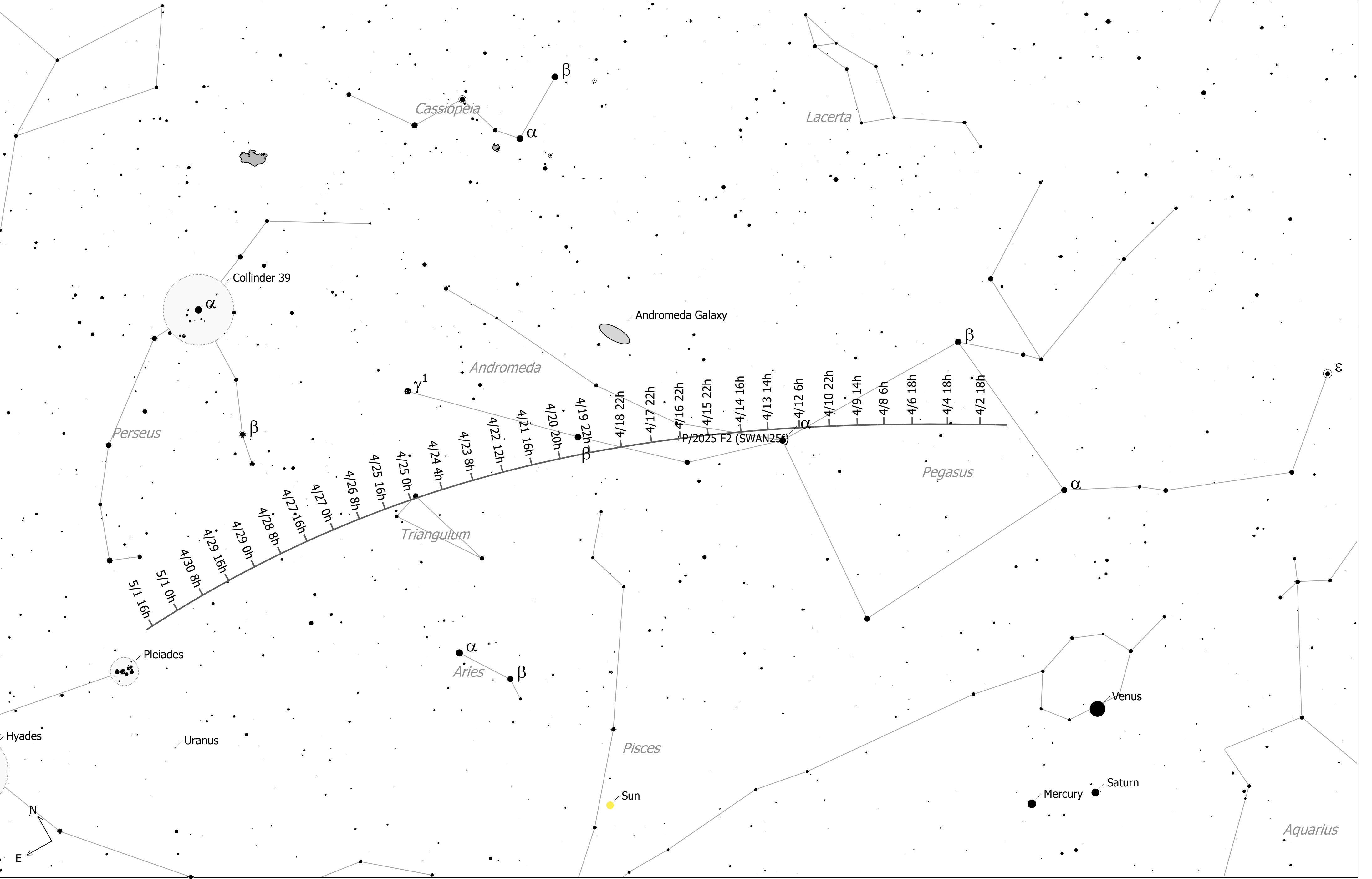
P/2025 F2 (SWAN25f) (Comet) Magnitude: 7.23 Coma Diameter: 2.5' SBr: 17.9 Mag/arcsec 2 Earth Distance: 1.2 AU
