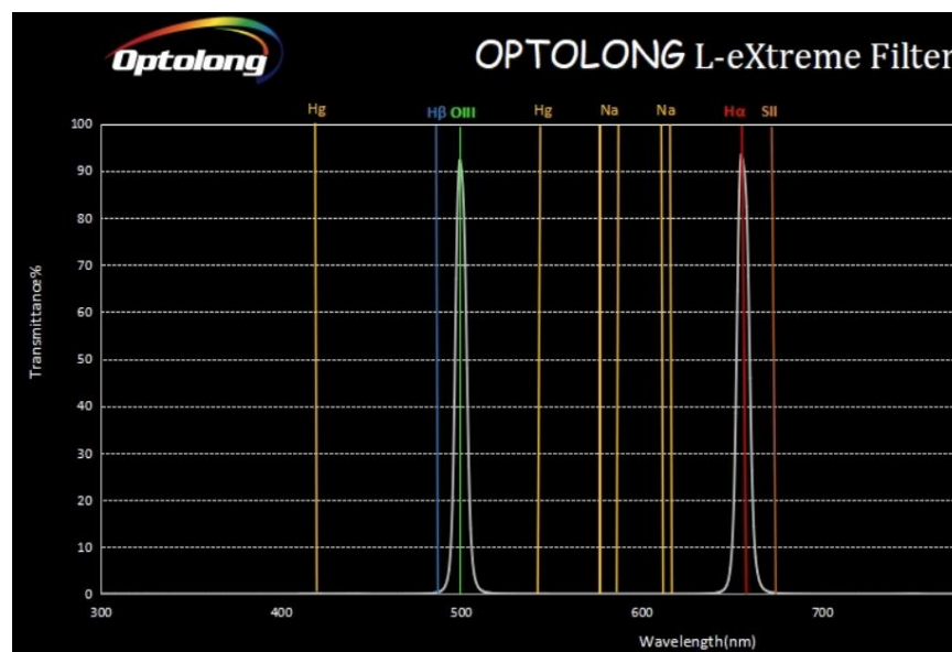
Narrow Band Filters Transmission Spectra
