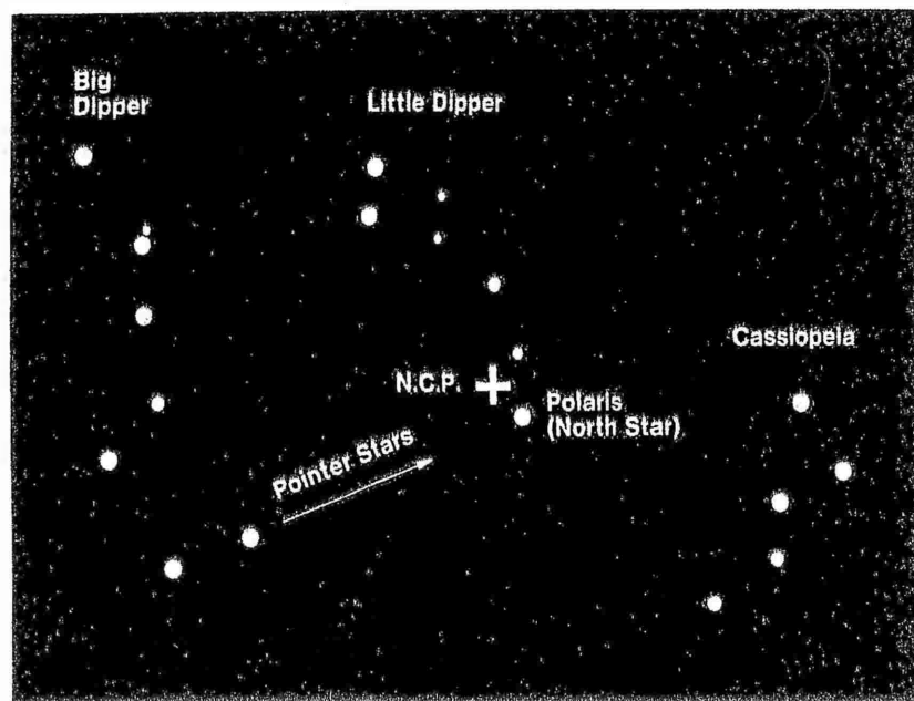
The Celestial Polar Region The two stars in the front of the bowl of the Big Dipper point straight to Polaris. Polaris is less than 1° from the true North Celestial Pole (N.C.P.). Cassiopeia is the "W" shaped constellation on the side of the pole opposite the Big Dipper. See "Lining Up on the Pole".
