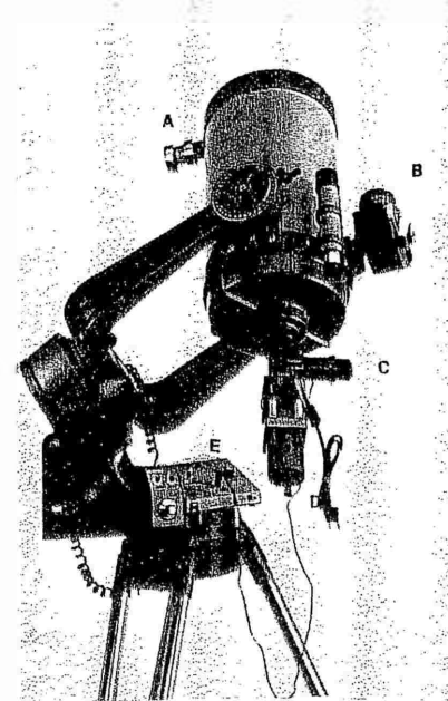
Astrophotography with the C8 (A) C8 counterweights (B) 35mm camera with lens on the piggyback mount (C) Off-axis guiding system (D) Cold camera (E) Drive corrector
