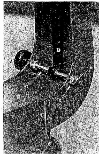
The Dec. Slow-Motion (A) Dec. slow-motion knob (B) Tangent arm (C) Tangent screw (D) Lock nut (E) Cone-point screw
