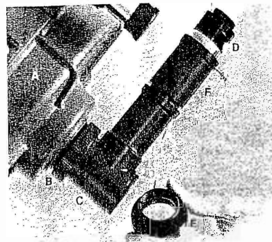
The Off-Axis Guiding System (A) Rear cell (B) Slip ring (C) Guider body (D) Illuminated reticle ocular. Also shown is the Tele-compressor (E) And its eyepiece extender (F).
