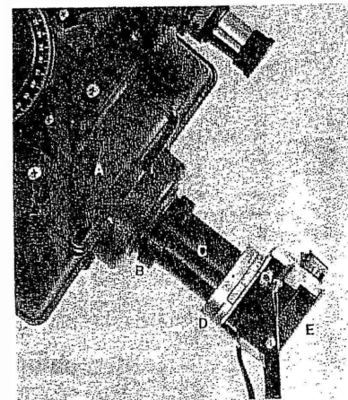
The T-Adapter (A) Rear cell (B) Slip ring (C) T-adapter (D) T-ring (E) Camera body
