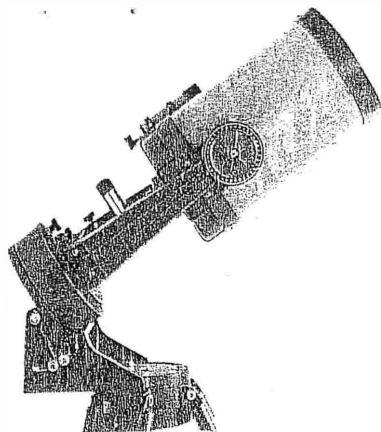
Polar Aligning on Polaris When the declination pointer reads 90°, the optical axis is parallel to the polar axis. At this setting, if Polaris is visible through the telescope, the polar axis of your Celestron is aligned on Polaris.
