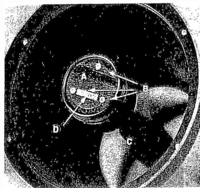
Collimation Adjusting Screws (A) Secondary mirror housing (B) Collimation adjusting screws (C) Schmidt corrector plate (D) Serial Number
