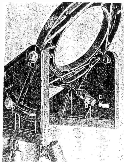
Adjusting the Wedge (A) Tilt plate (B) Adjusting screw (C) Latitude adjuster (D) Tilt plate bolts (on both sides of wedge)
