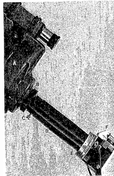
The Tele-Extender (A) Rear cell (B) Visual back (C) Set screw (D) Tele-extender (E) T-ring (F) Camera body
