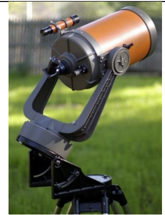
Schmidt-Cassegrain on Fork Mount with Wedge and Clock Drive
