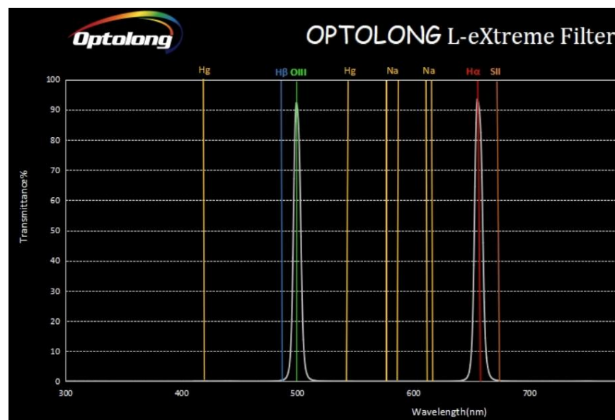
Narrow Band Filters Transmission Spectra
