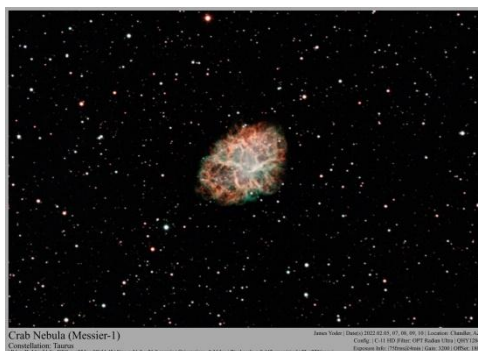
M-1: Supernova Remnant
