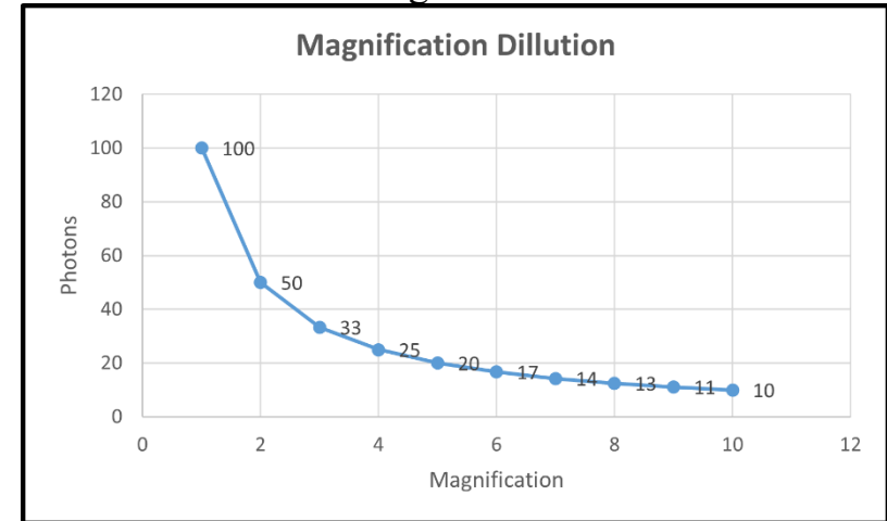
Chart 4.3: Magnification Dilution
